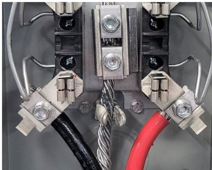
Figure 17 – Split-Bolt Connector Main/Run
