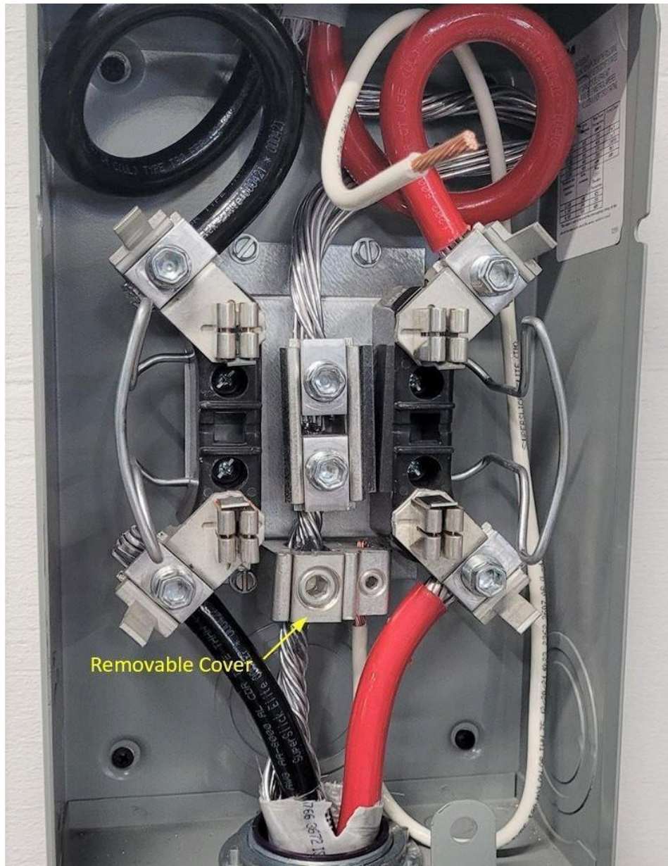
Figure 15 – Parallel Tap Connection
