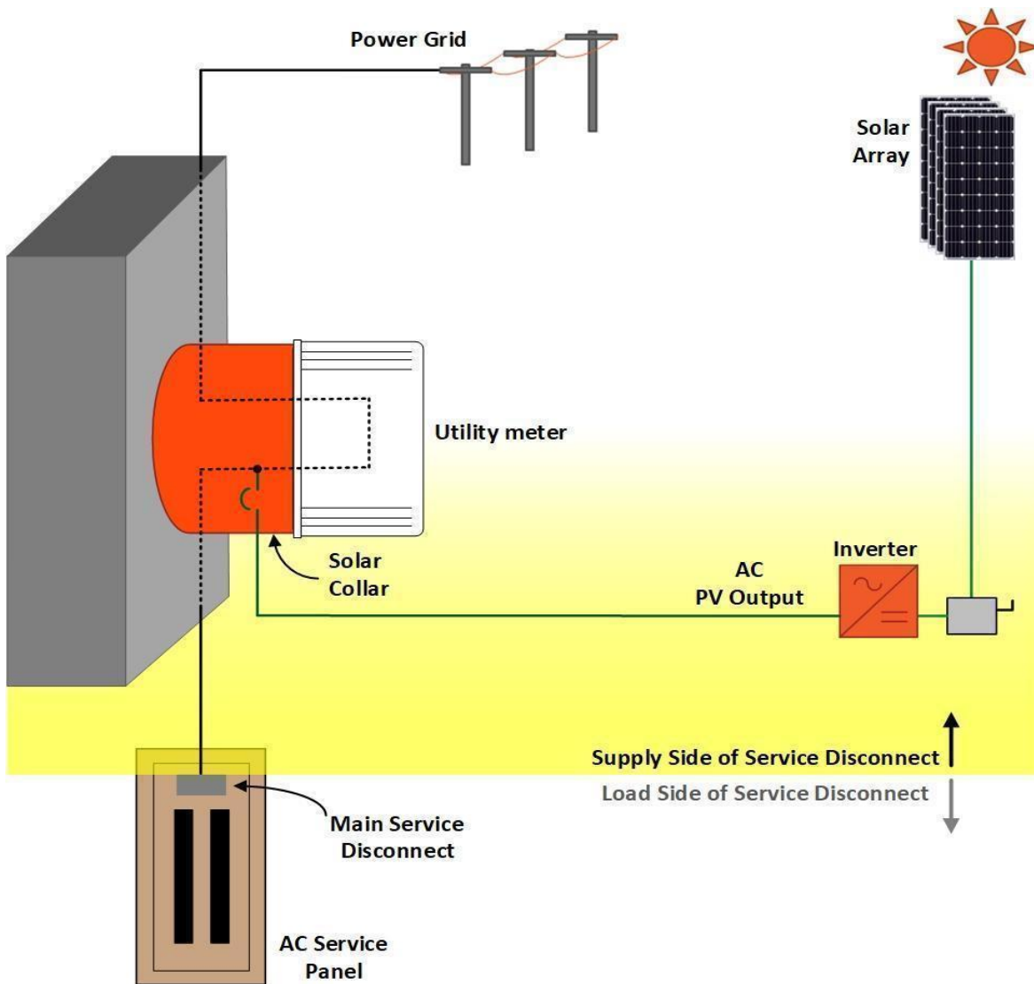
Figure 2 – Conceptual Supply-Side Solar PV Interconnection
